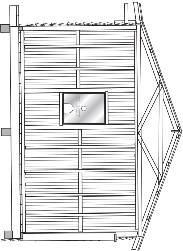
Cross Sections of waiting room B - B
